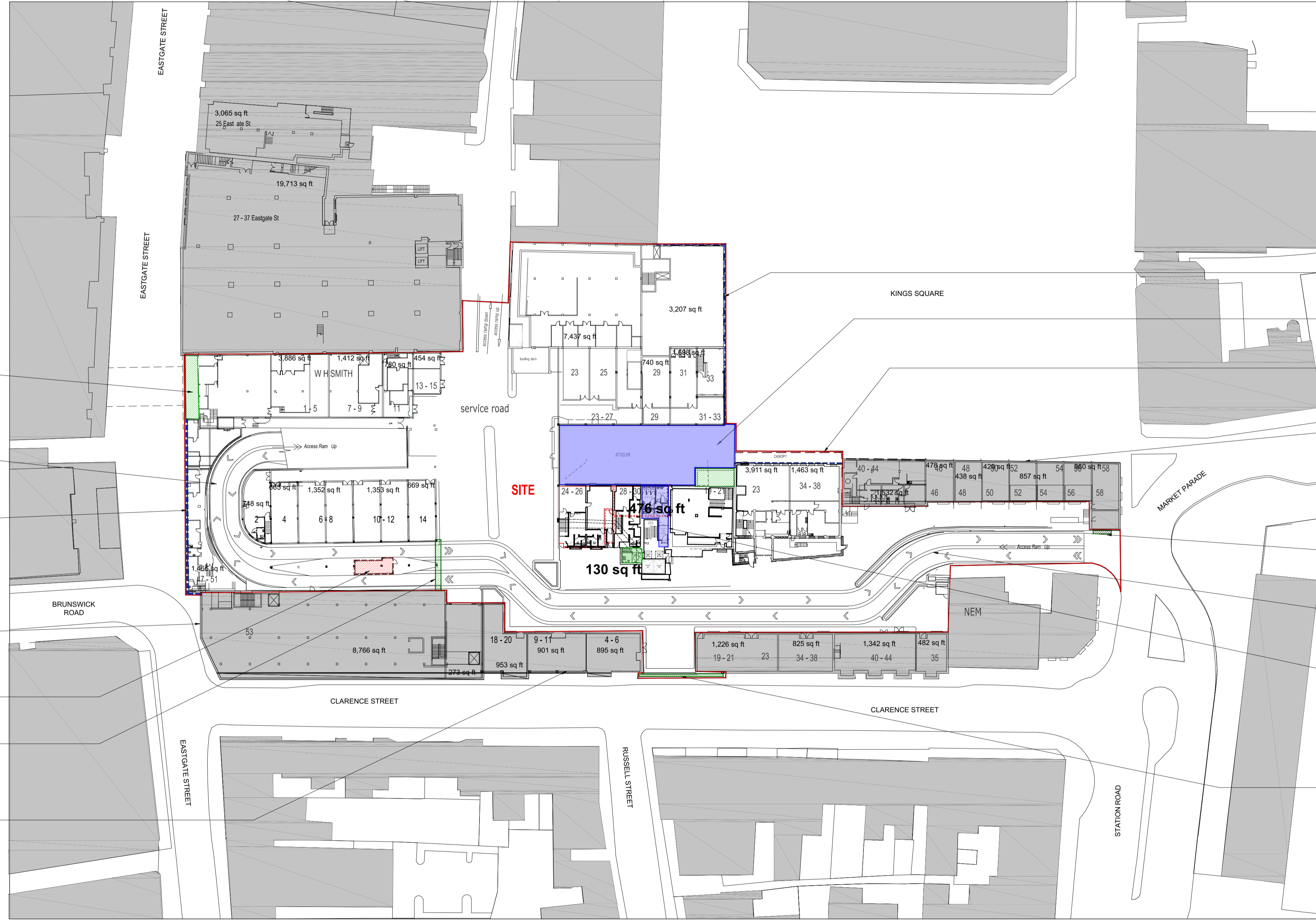
PROPOSED FIRST FLOOR BLOCK PLAN 1:500
